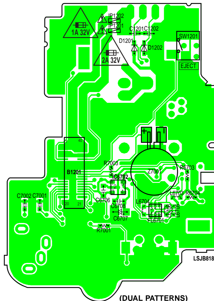
(FOIL SIDE)
